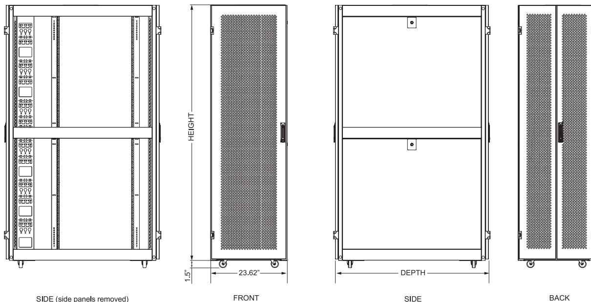
SIDE (side panels removed)
