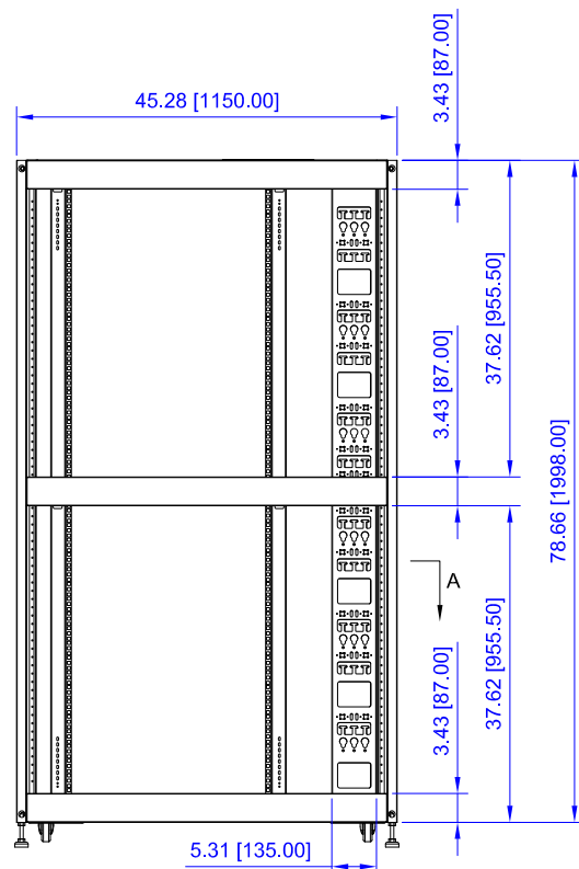
SIDE VIEW (NO SIDE PANELS)
