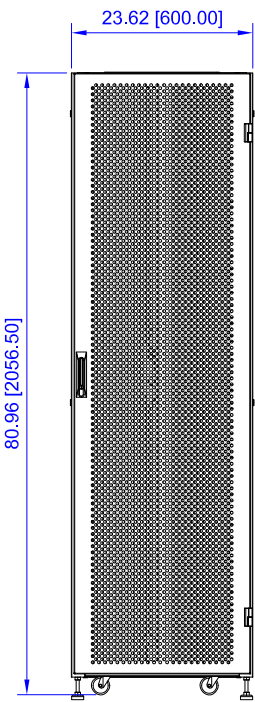
FRONT VIEW
