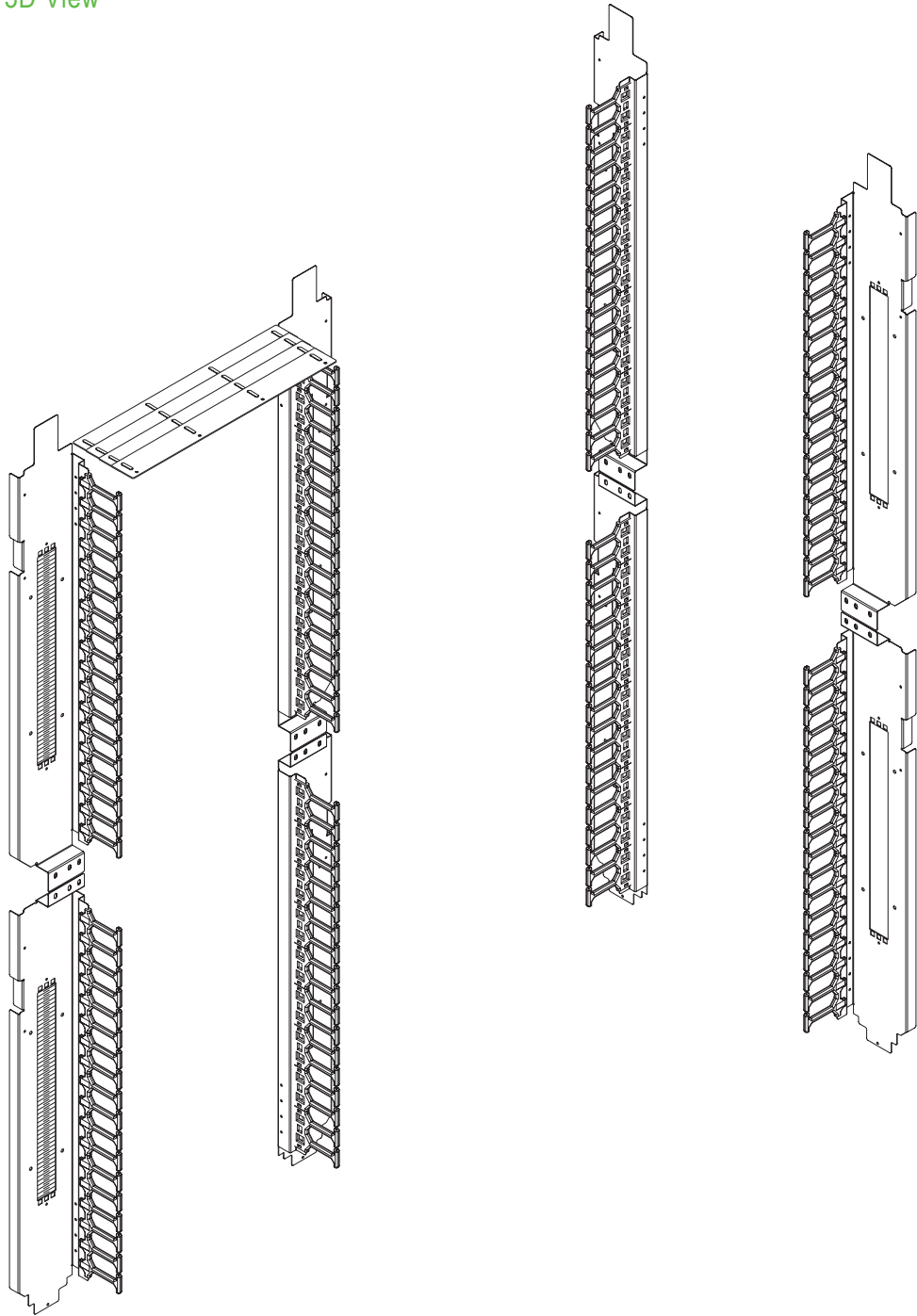
Technical Drawing- 3D View
